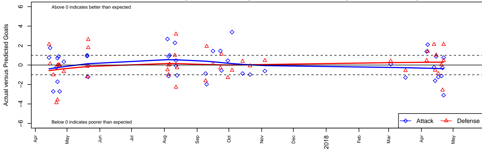
Sting SC Timbers Red B05 Dots are actual minus expected GF (blue circles) and GA (red triangles). Blue line is smoothed change in attack strength. Red is smoothed change in defense strength.
